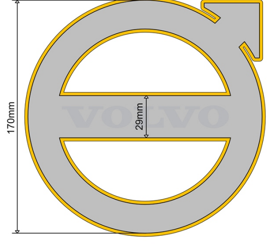
Original emblem dimensions
